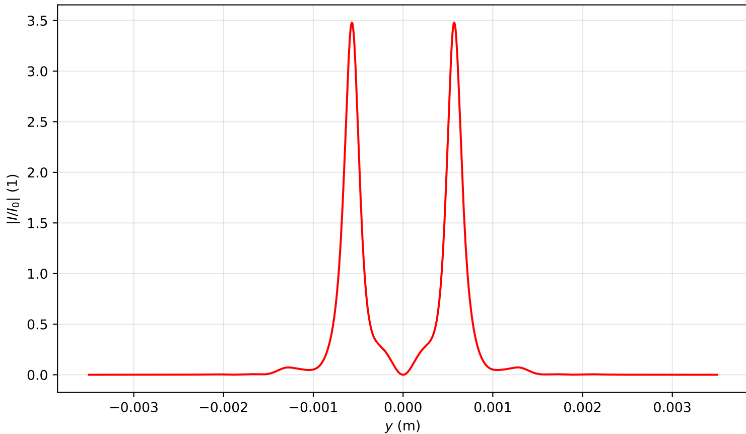
Intensity profile I(x=0, y, z=1.115)/I_0 , \text{Pin}=9.0\text{Pcr} , artificial time
